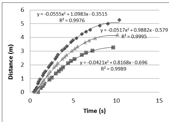
Figure 9: Friction Measurement
