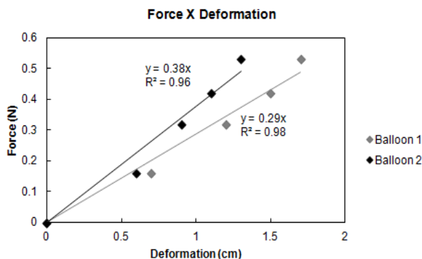
Figure 5: chart of the applied force versus deformation of the balloon strip.
