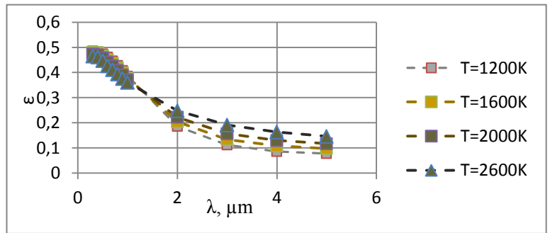
Figure 5. Diagram plotting emissivity of tungsten against wavelength for different temperature.
