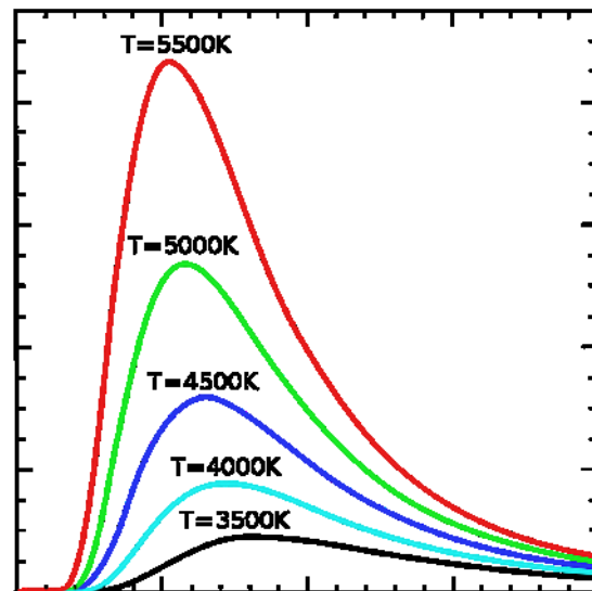
Figure 4. Diagram plotting Planck’s Law 3 for blackbody of different temperature. Plot: spectral density of radiant emission against a wavelength.
