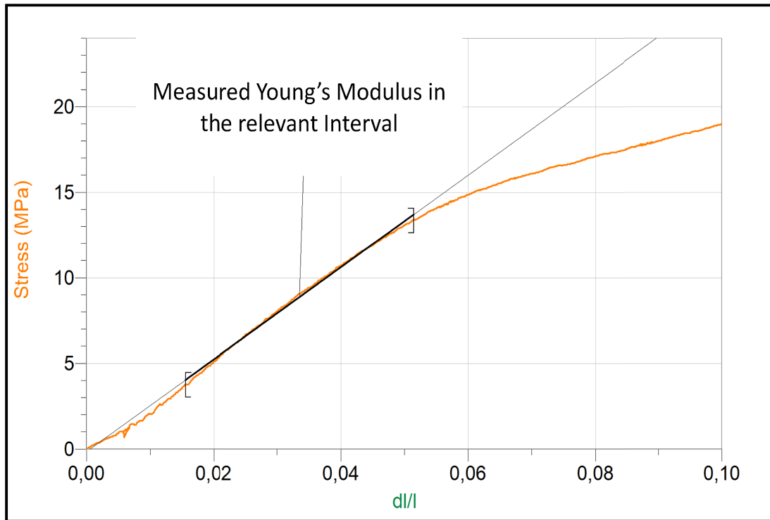
Figure 5: Stress-strain curve of the Nopi ® - Tape
