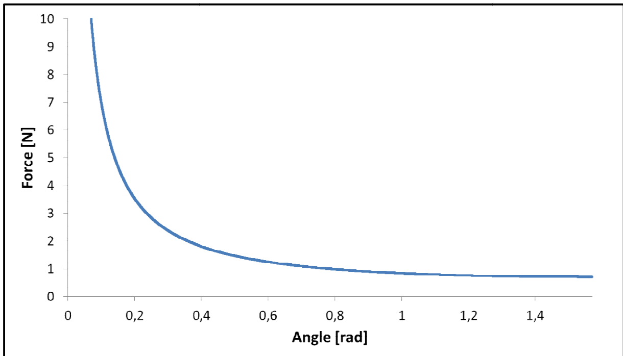
Figure 8: Plot of the critical force to pull of the Nopi ® – Tape in dependence on the angle
