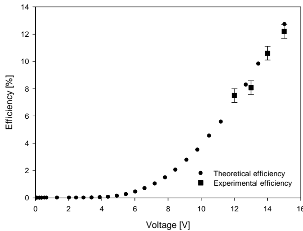
Graph 4. Efficiency-voltage dependence
