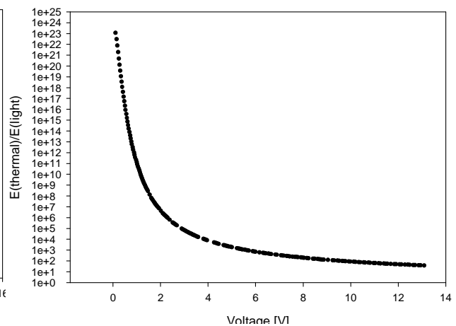
Graph 5. Ratio P_{IR}/P_V -voltage dependence (real light limits)
