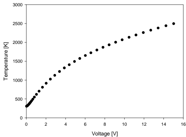
Graph 2. Temperature-voltage dependence
