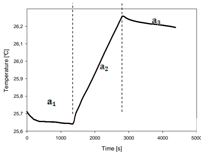
Graph 1. Temperature-time dependence
