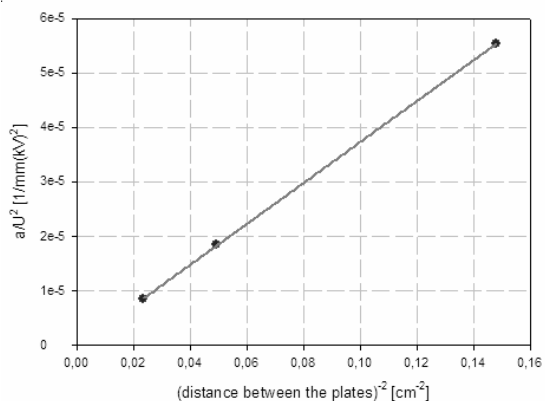
Graph 3: coefficient of lines from previous graph b; in dependance of distanced from plate
