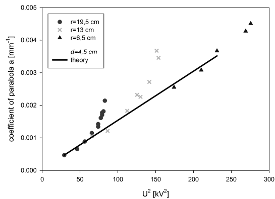
Graph 4: coefficient of parabola a doesn't depend on the radius of soap film
