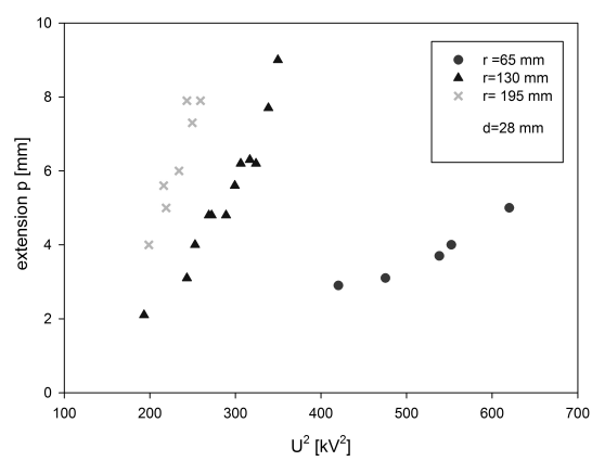
Graph 7: dependence of extension p on voltage for different radius of soap film
