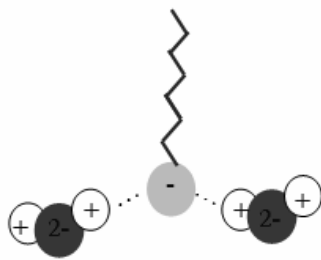
Figure 1: Soap molecule
