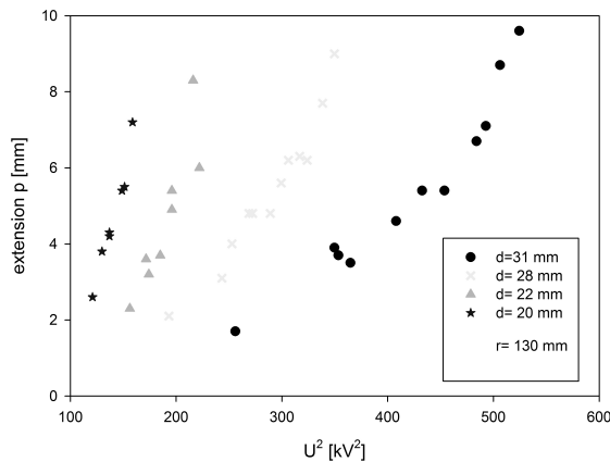
Graph 6: dependence of extension p on voltage for different distance from steel ball
