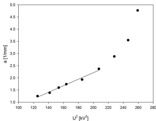
Graph 1: coefficient of parabola a in dependance of voltage
