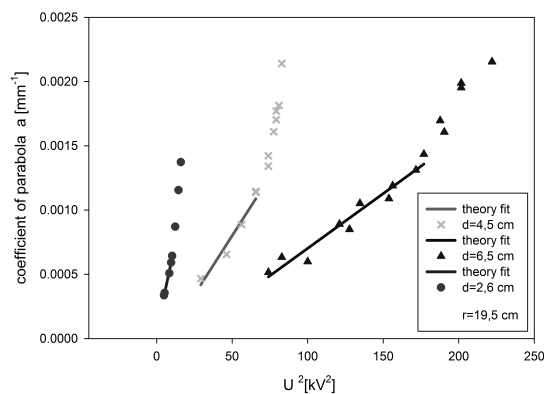
Graph 2: coefficient of parabola a in dependance of voltage for different distanced from plate
