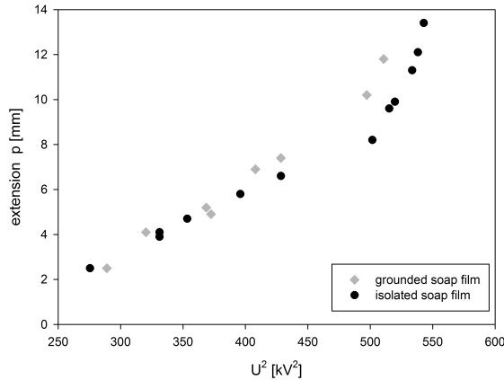
Graph 5: extension p for grounded and isolated soap film
